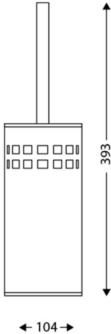
TECHNICAL DRAWING
