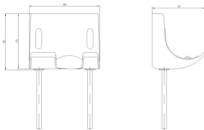
TECHNICAL DRAWING
