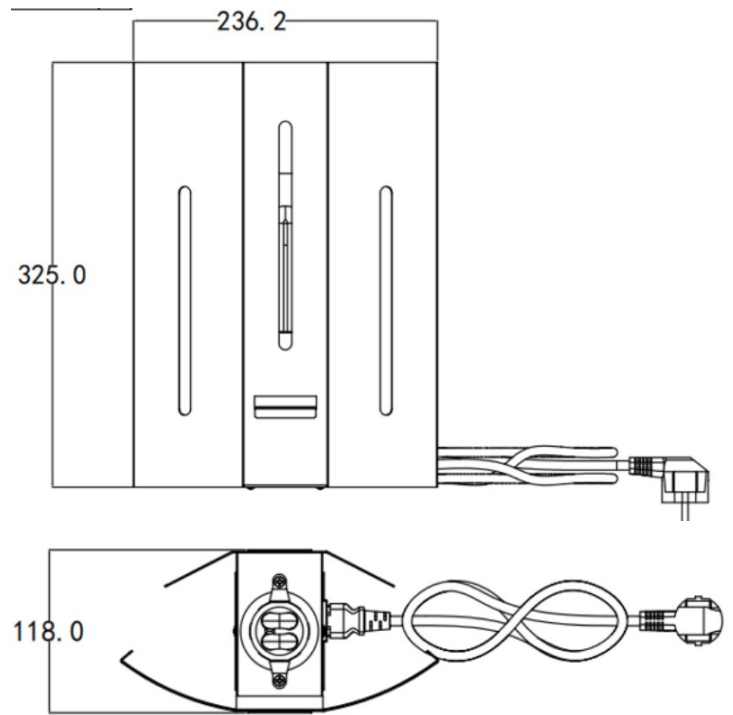
TECHNICAL DRAWING
