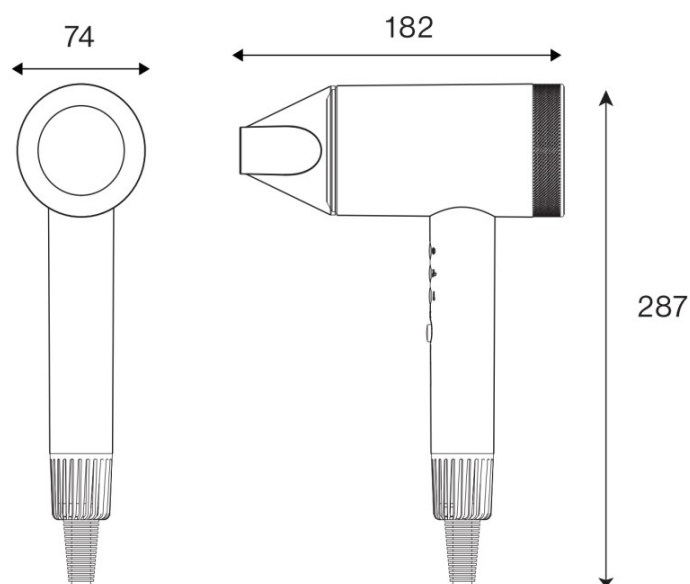
TECHNICAL DRAWING
